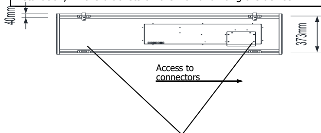
Rear view of the display with mounting brackets.
